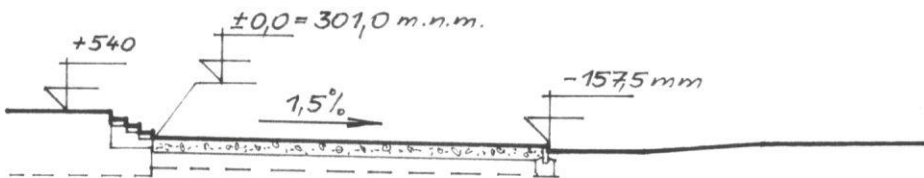
REZ 2-2; M = 1:200
