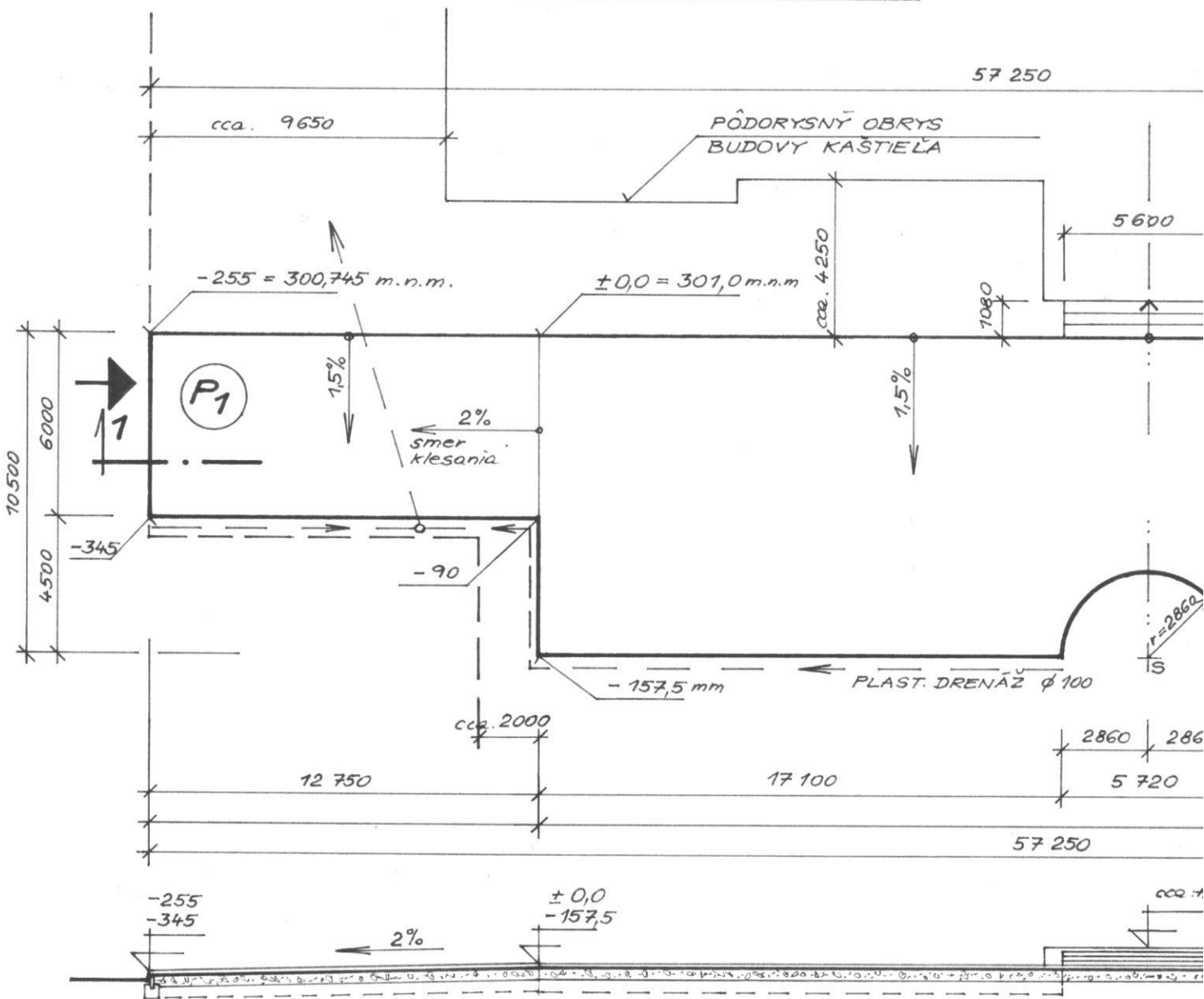
REZ 1-1; M = 1:200
